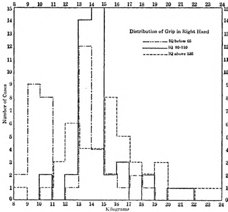
FIG. 17 (Part II). — Showing comparative distribution of right-hand grip, in kilograms, of three groups of children, 9 to 11 years old — age, sex, and race being constant in the three groups. (From "Size and Strength of Children Who Test above 135 IQ" by Hollingworth and Taylor. Reproduced, by courtesy of The National Society for the Study of Education, from The Twenty-Third Yearbook .)
